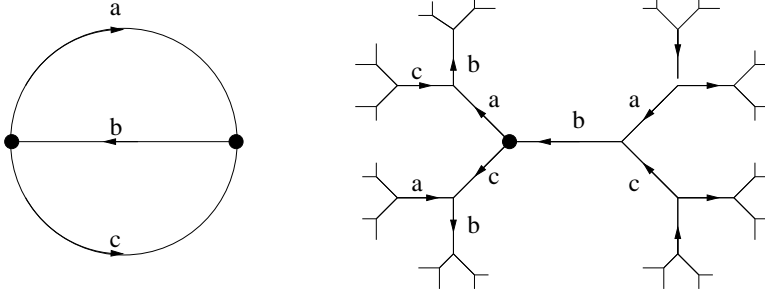
FIGURE 8: GENUS TWO: SECOND CASE.
