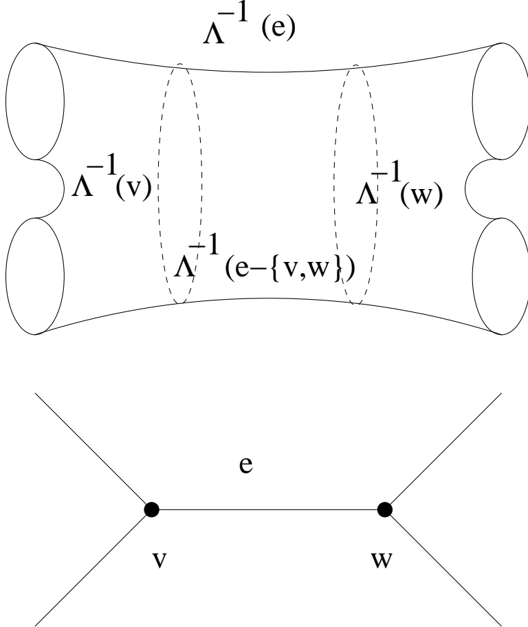
FIGURE 11: THE p -ADIC UPPER HALF-PLANE AND THE BRUHAT–TITS TREE.
