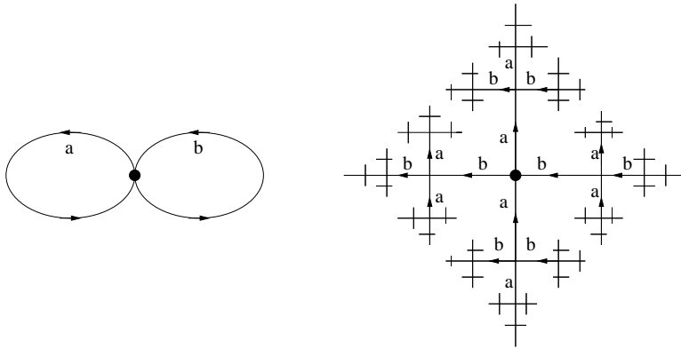
FIGURE 7: GENUS TWO: FIRST CASE.
